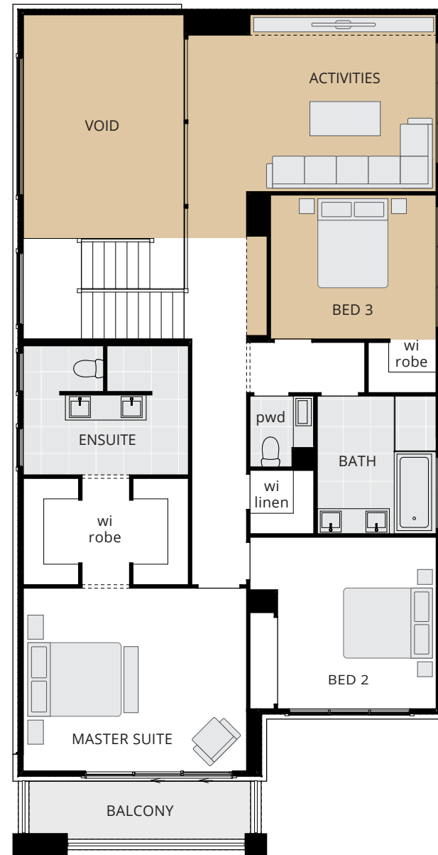
FIRST FLOOR
